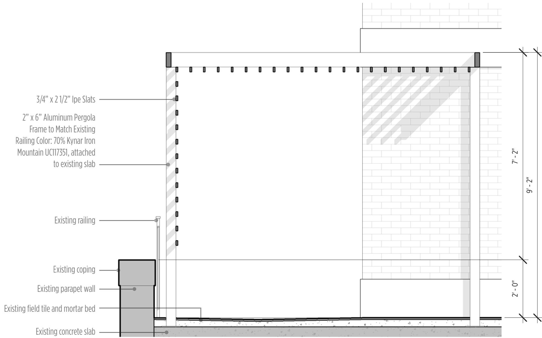
PERGOLA SECTION
